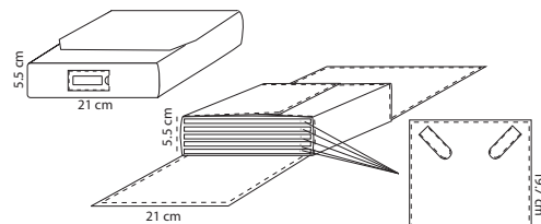
cod. VRO00055 ( 5 inserts for necklaces)
