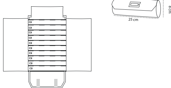
cod. VRO00035 ( 10 spaces for necklace with bottoms )
